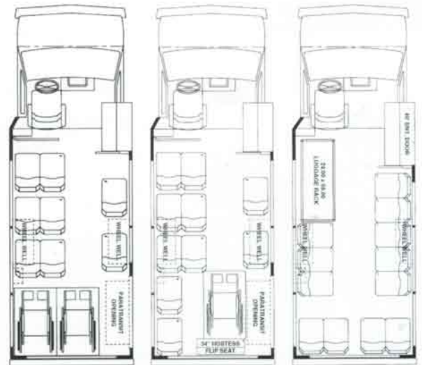
MODEL CR210, 10 Passenger, Rear Lift
