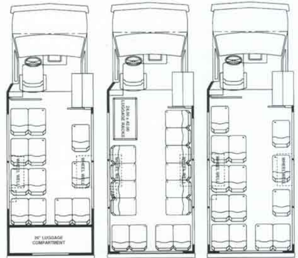
MODEL CR210, 12 Passenger, Rear Luggage
